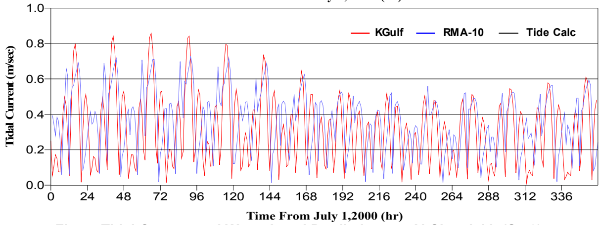
Fig. 7. Tidal Current and Water Level Predictions at Al-Shuwiakh (St. 3).
